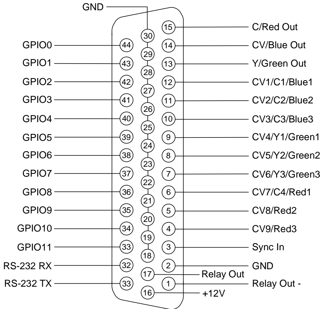
HD-22 44-Pin Female AMP 5748482-5
